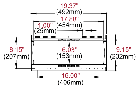
WALL PLATE
