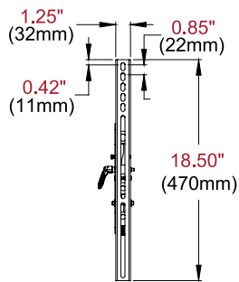
VERTICAL ADAPTOR
