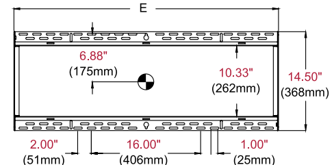
WALL PLATE DETAIL
