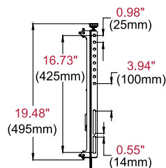
ADAPTOR BRACKET DETAIL
