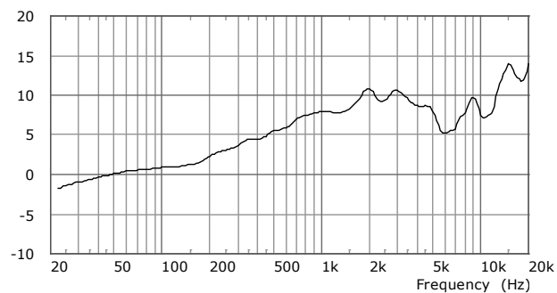
Directivity Index (DI)
