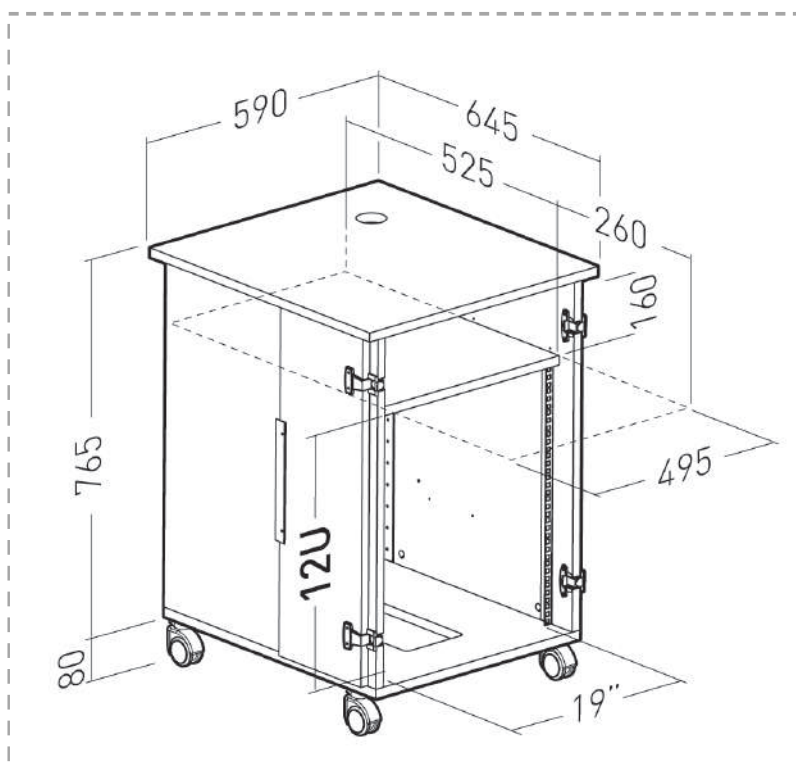
WOODY 12U (ref. 777000 - ref. 777002 - ref. 777003 - ref. 777008)
