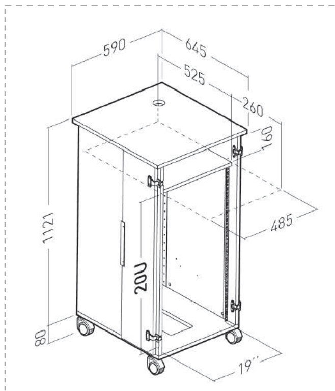
WOODY 20U (ref. 777001)
