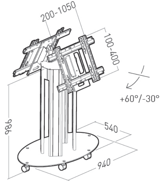
MOBILE / MOBILE
