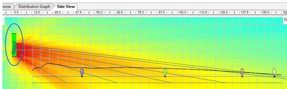
Figure 13. With defined height limits showing (green column), move the array up/down (+ Auto Splay each time) to find best coverage
