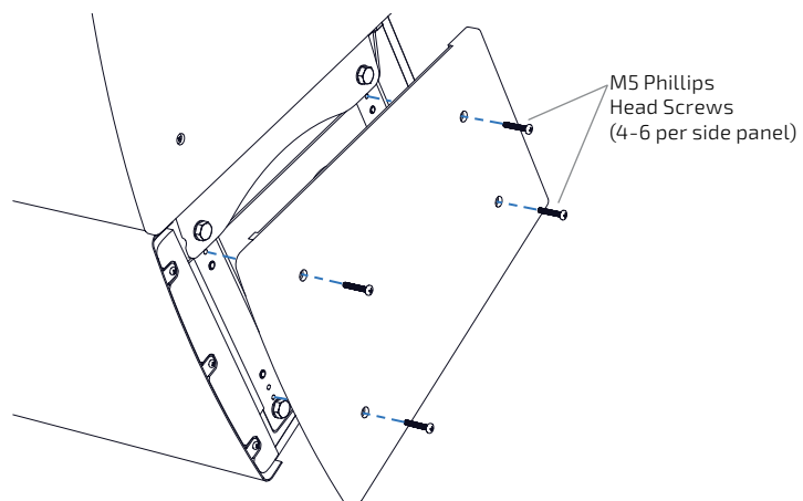
Figure 4. Attach side panels after all bracket connections / hardware has been installed
