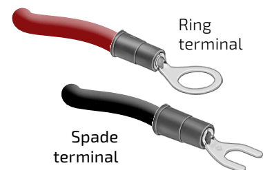
Figure 26. Wire connectors
