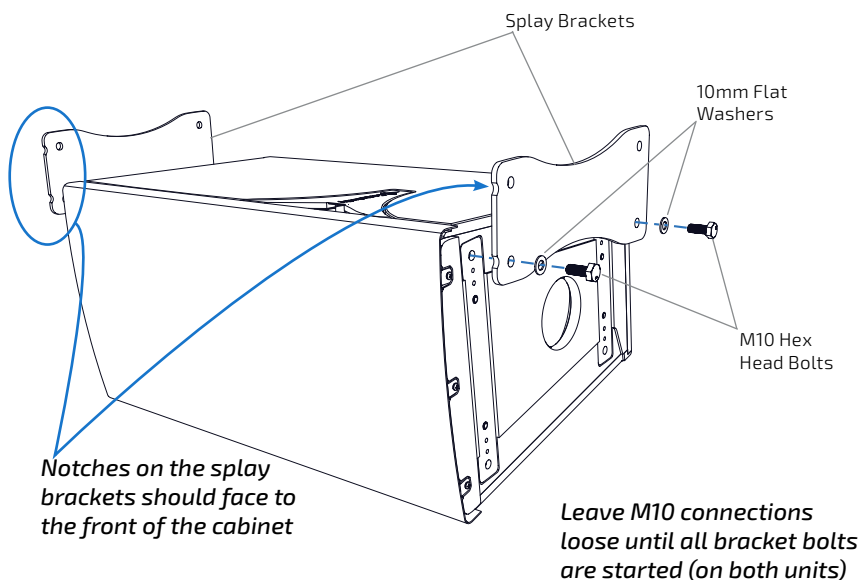
Figure 1. Typical splay bracket attachment to a cabinet
