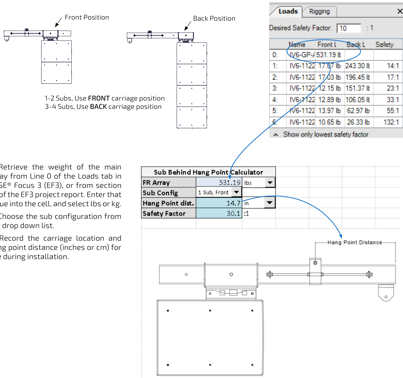
Figure SB. Sub Behind Hang Point Calculator
