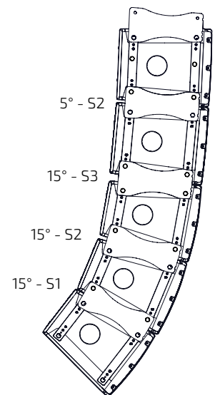
Gradual Curve 5° and 15° with splay brackets
