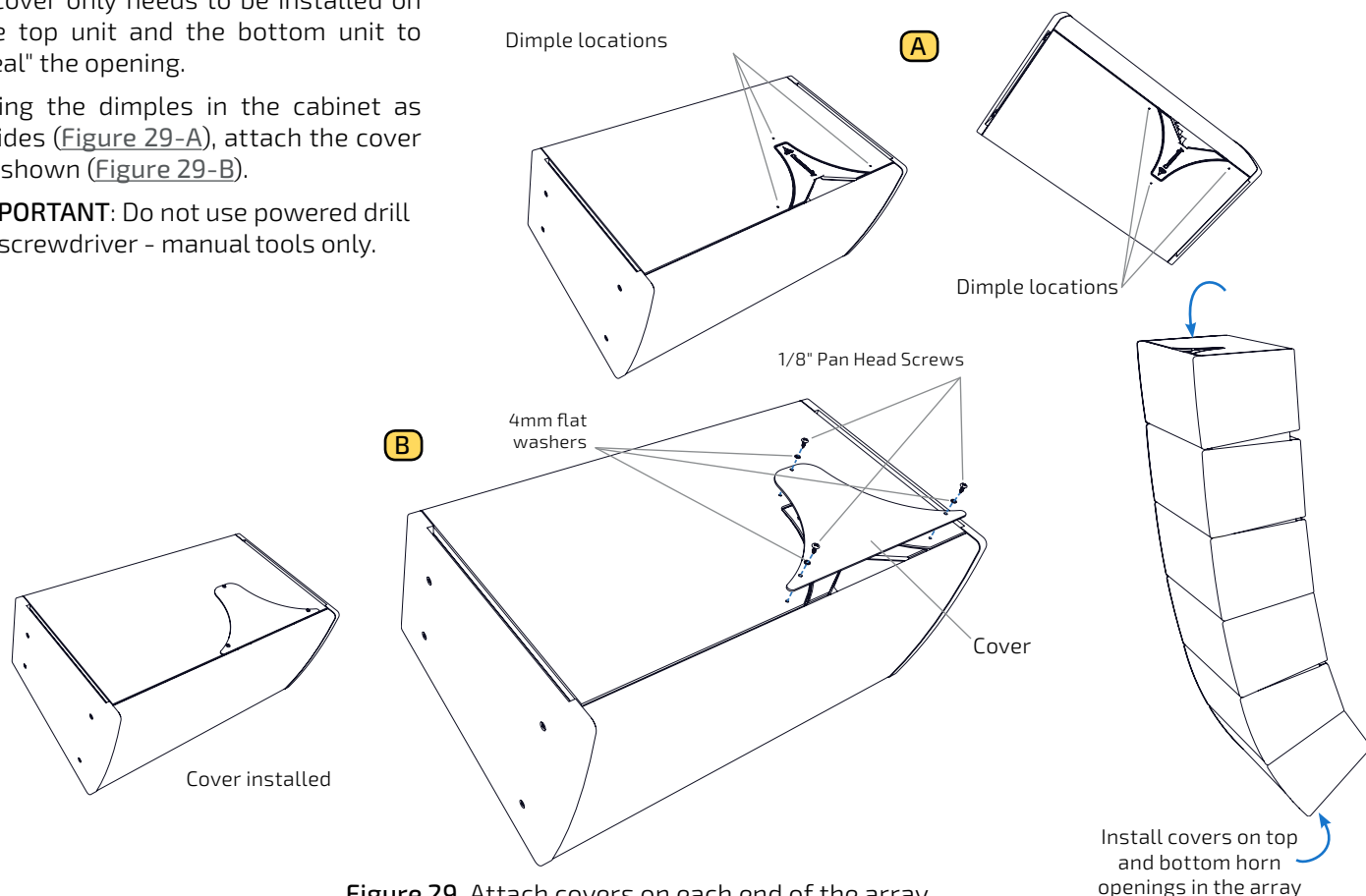
Figure 29. Attach covers on each end of the array A. Dimple locations B. Cover attachment
