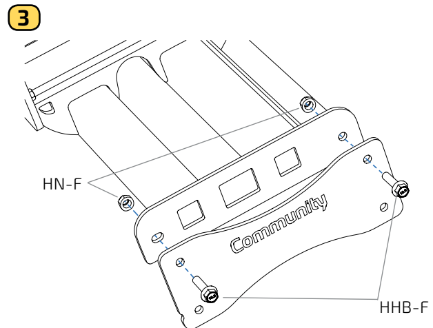
Step GP-3. Using the 10.9 hardware, loosely connect the splay brackets to the array frame with "Community" facing out
