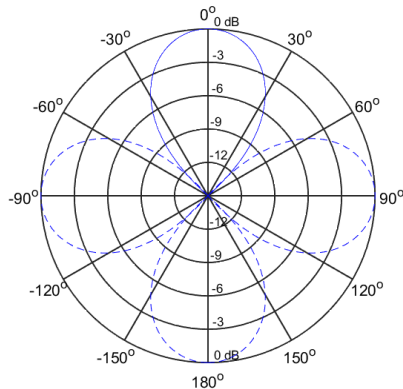
BEAMFORMING RANGE Polar Pattern Shown at 2000Hz at an elevation of 30°
