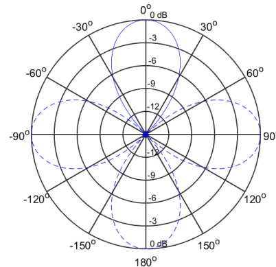
BEAMFORMING RANGE Polar Pattern Shown at 4000Hz at an elevation of 30°
