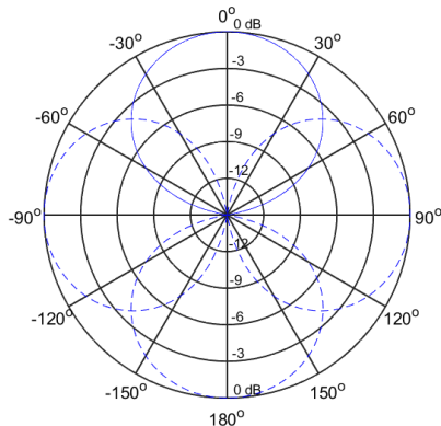
BEAMFORMING RANGE Polar Pattern Shown at 1000Hz at an elevation of 30°
